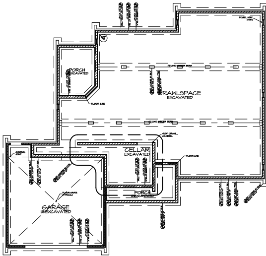
1 FOUNDATION PLAN A-2
