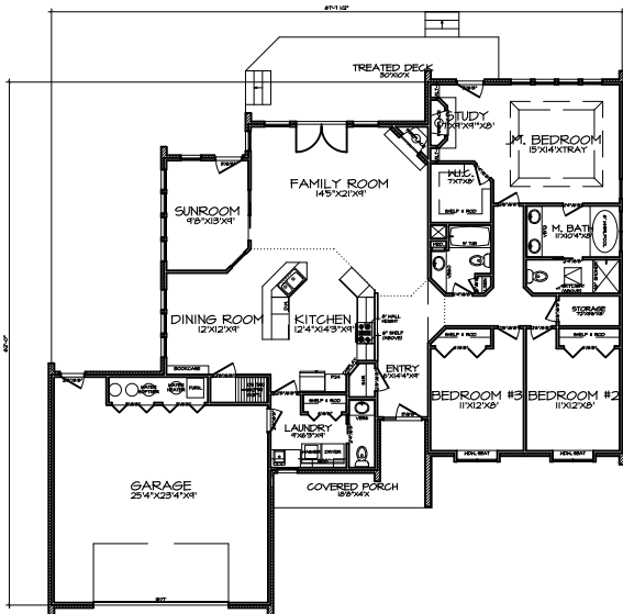
1 FIRST FLOOR PLAN A-3
